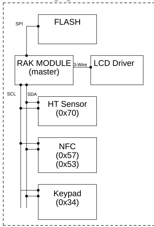
SPI_I2C_CONNECTIONS
