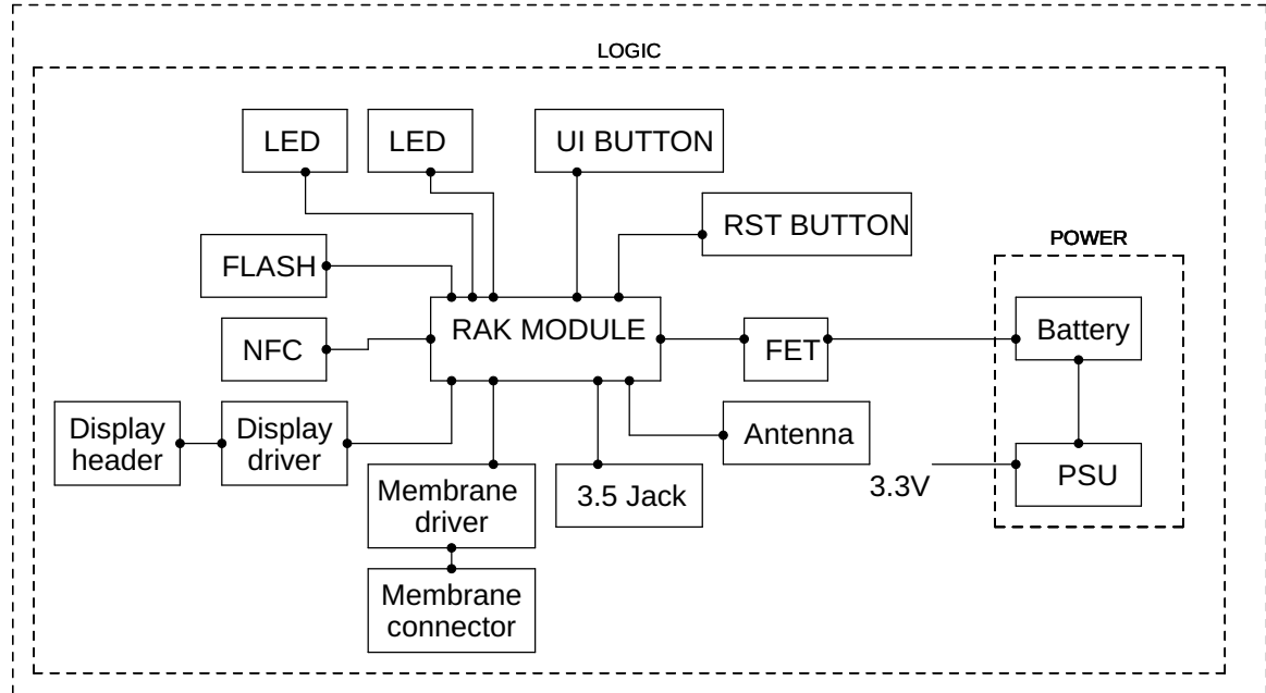
BLOCK DIAGRAM
